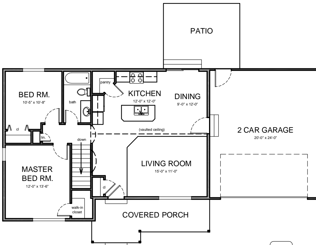
FIRST FLOOR LEVEL
