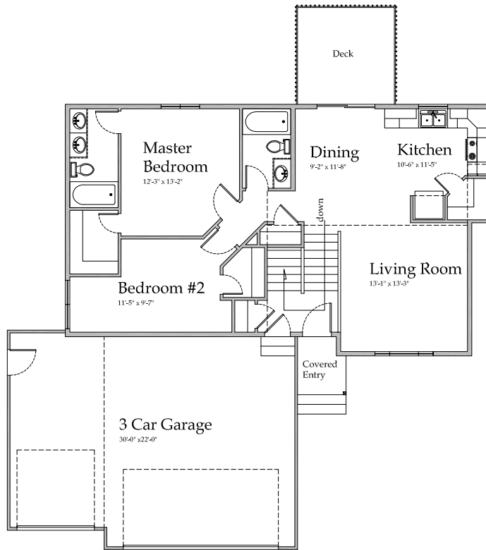
Main Floor
