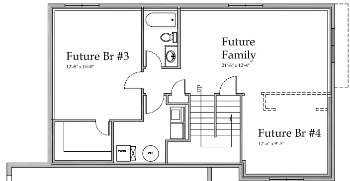
Lower Floor
